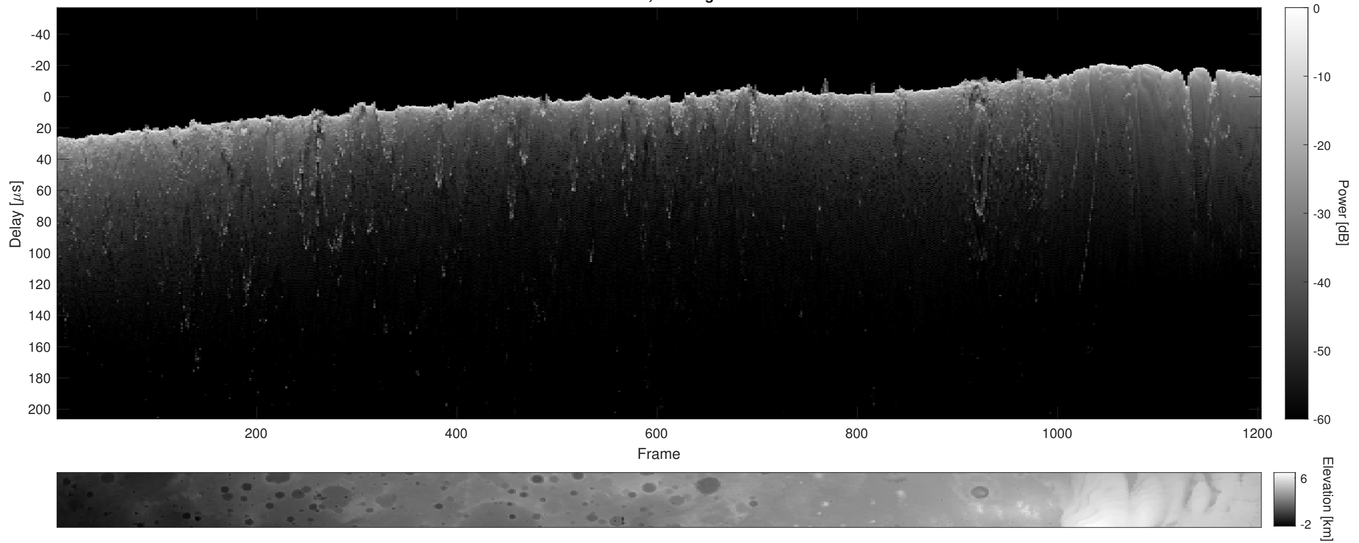
Orbit 4828, Cluttergram
