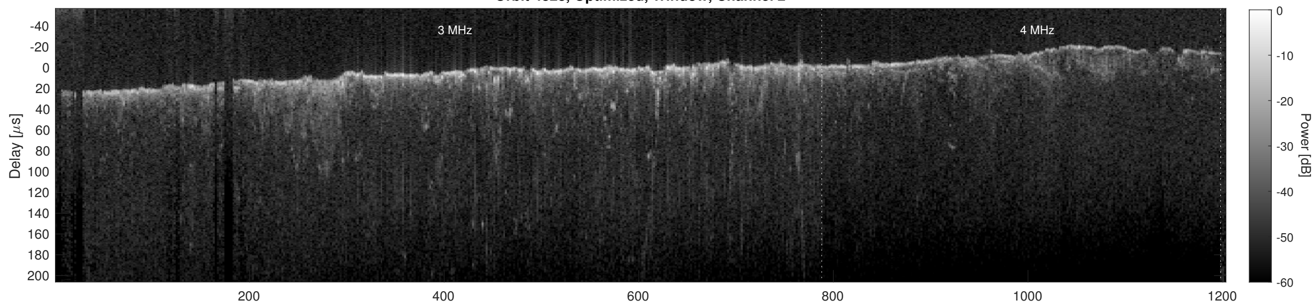
Orbit 4828, Cluttergram
