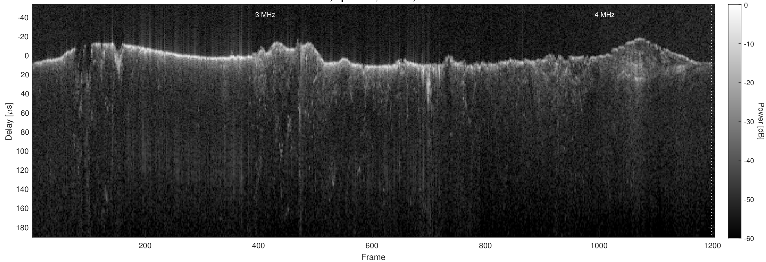
Orbit 4829, Optimized, Window, Channel 2
