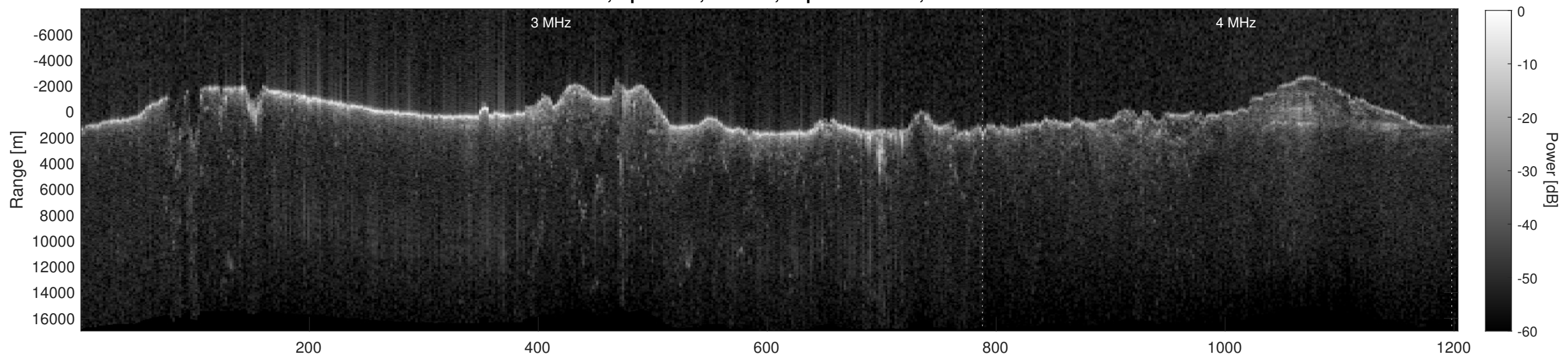
Orbit 4829, Depth-Corrected Cluttergram
