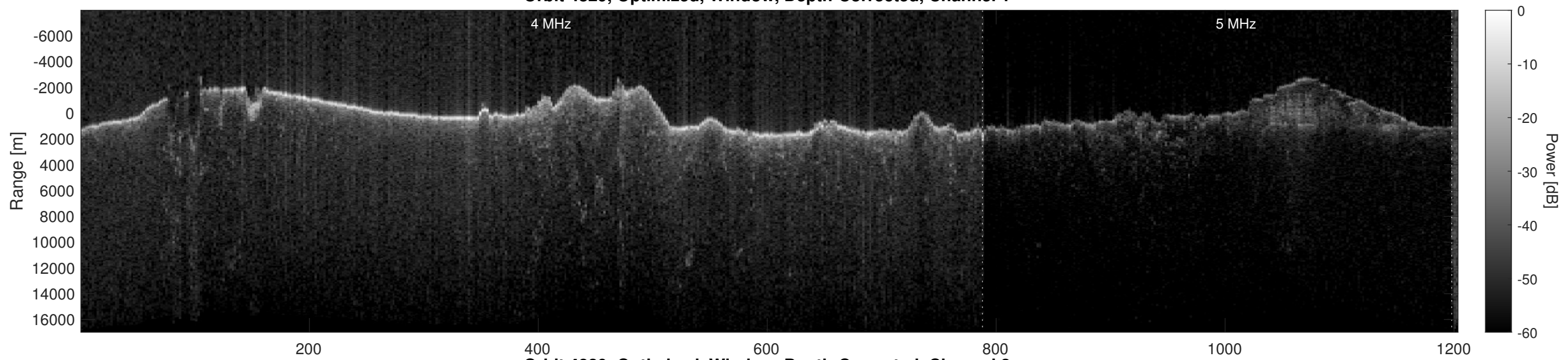
Orbit 4829, Optimized, Window, Depth-Corrected, Channel 2
