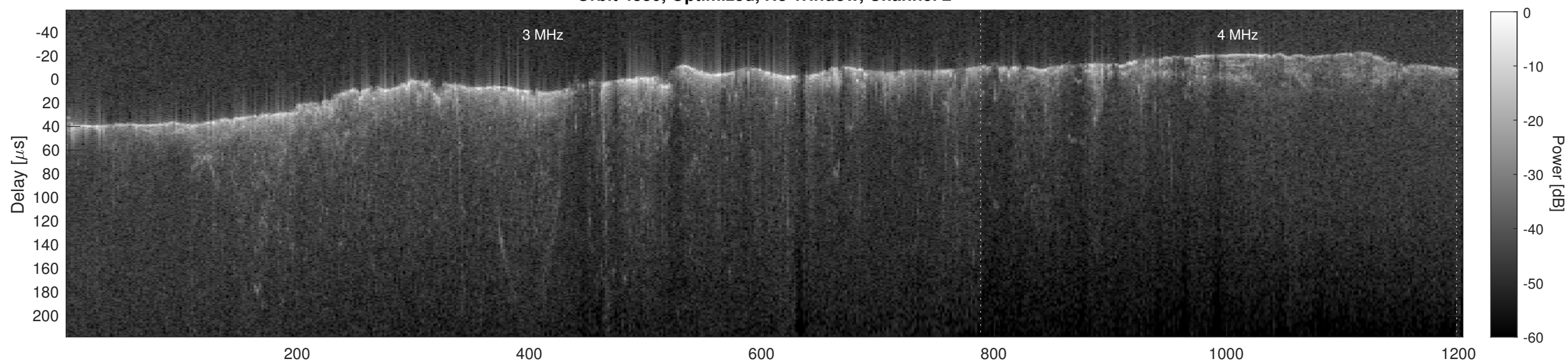
Orbit 4830, Cluttergram
