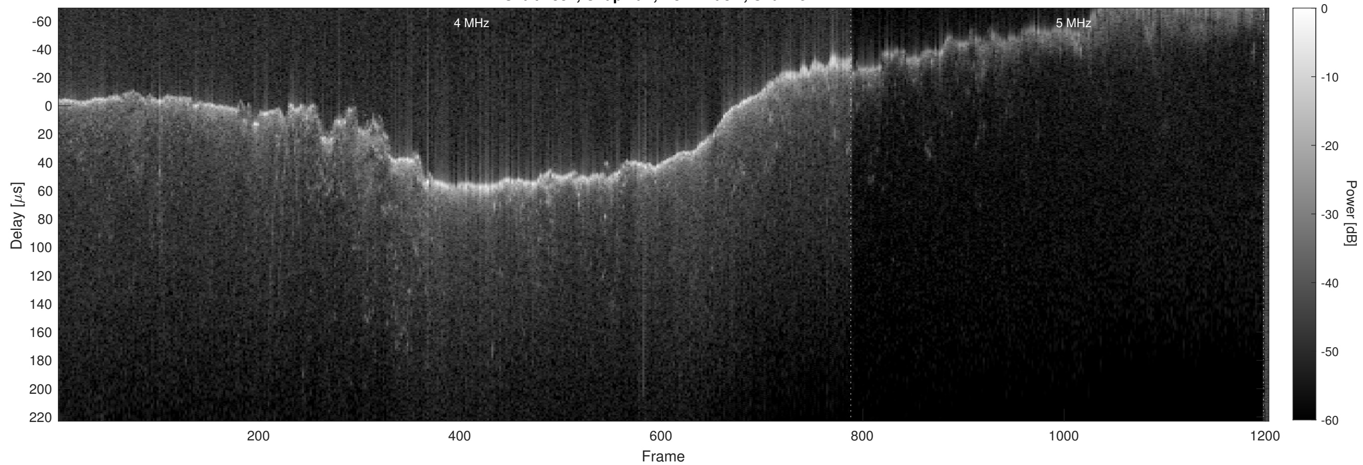
Orbit 4831, Chapman, No Window, Channel 2
