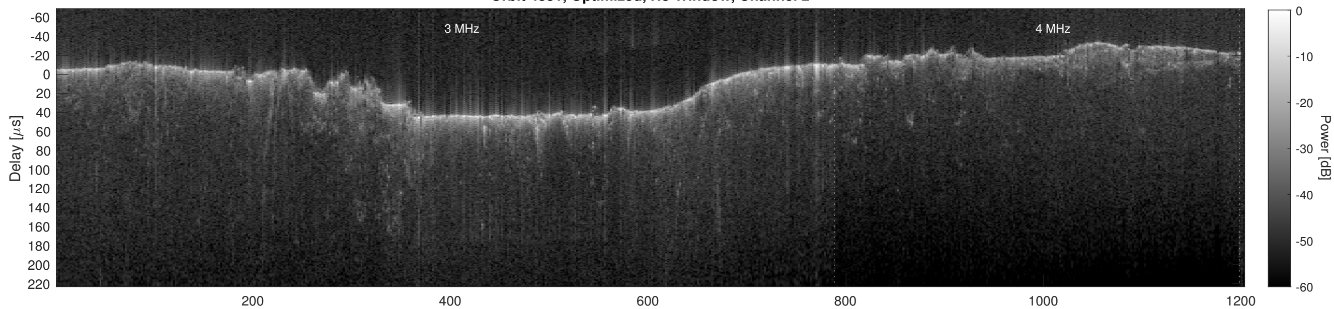
Orbit 4831, Cluttergram
