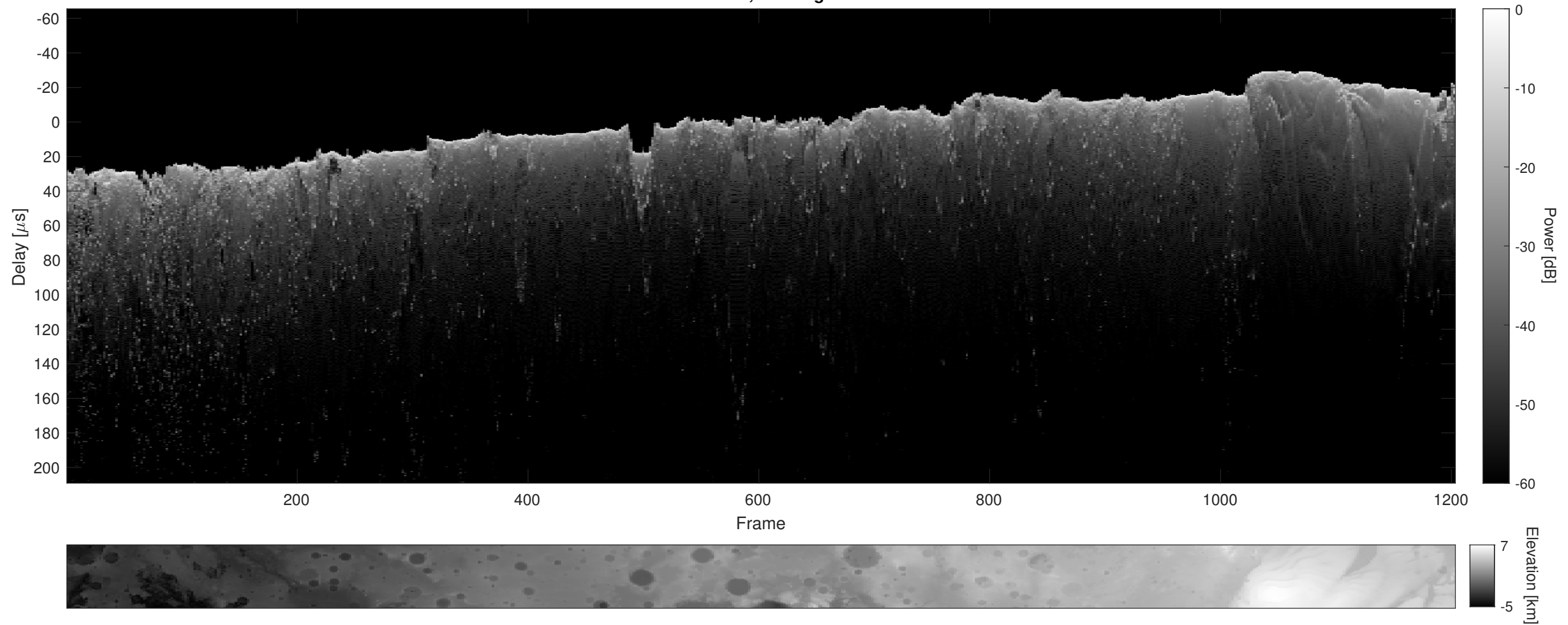
Orbit 4832, Cluttergram
