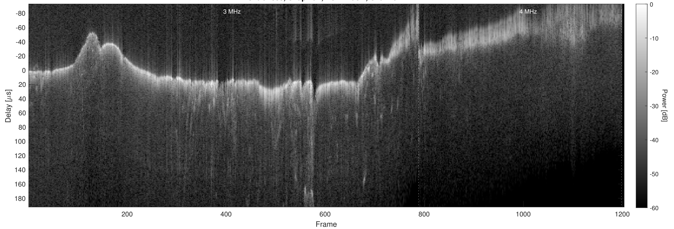
Orbit 4833, Chapman, No Window, Channel 2
