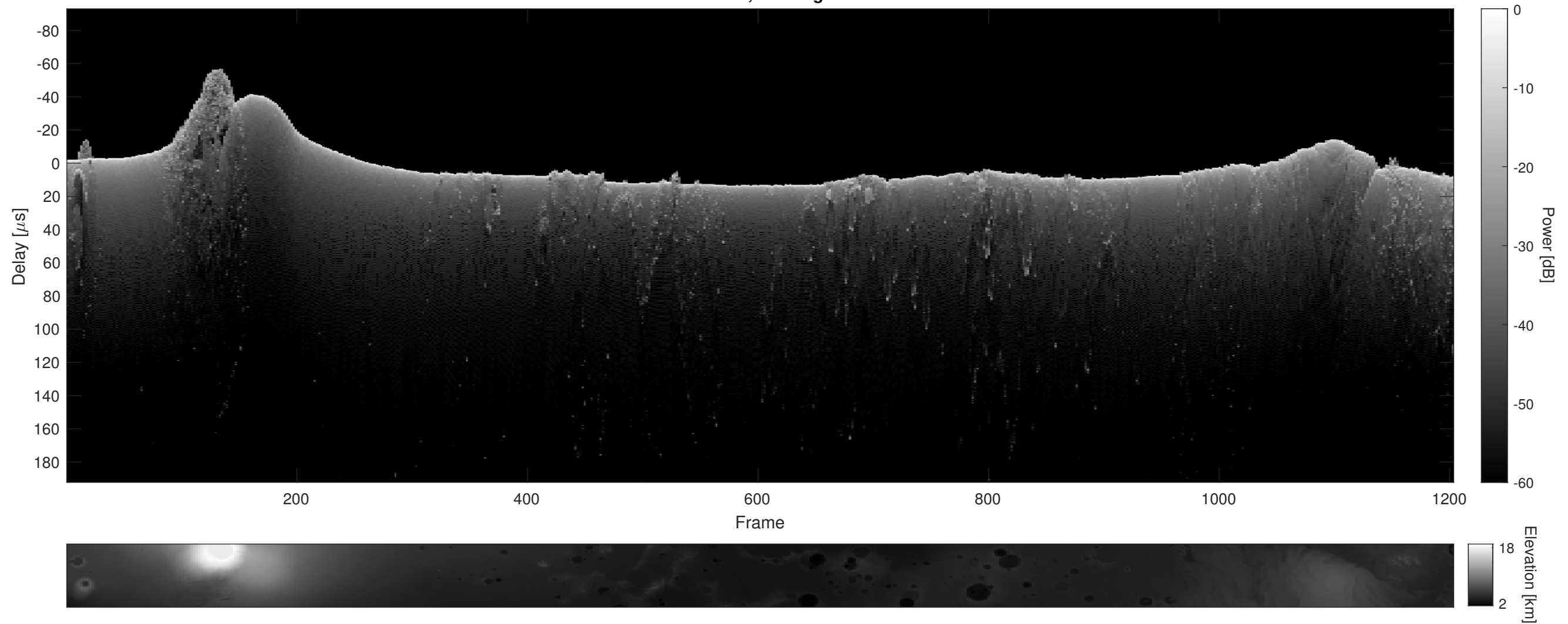
Orbit 4833, Cluttergram
