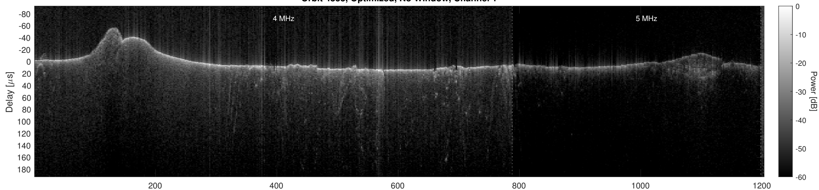
Orbit 4833, Optimized, No Window, Channel 2
