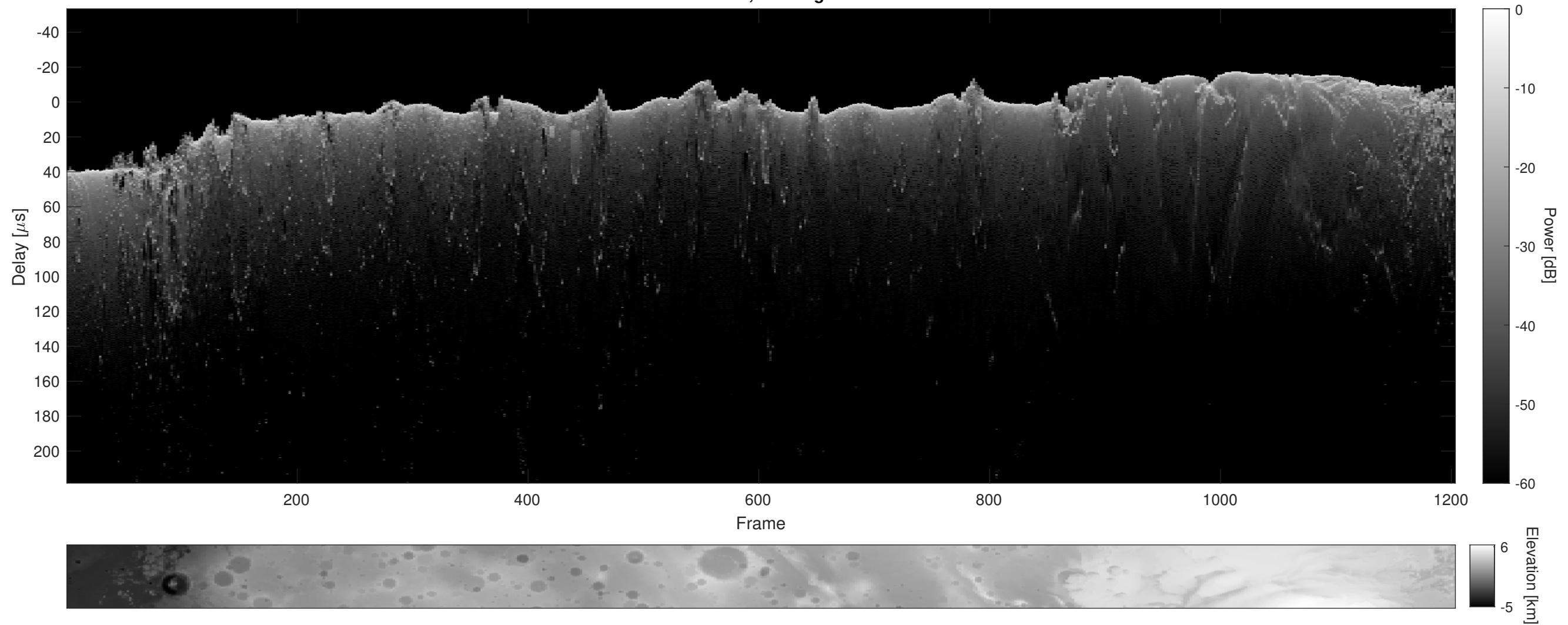
Orbit 4834, Cluttergram
