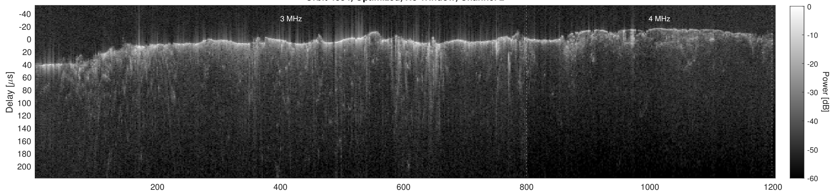
Orbit 4834, Cluttergram
