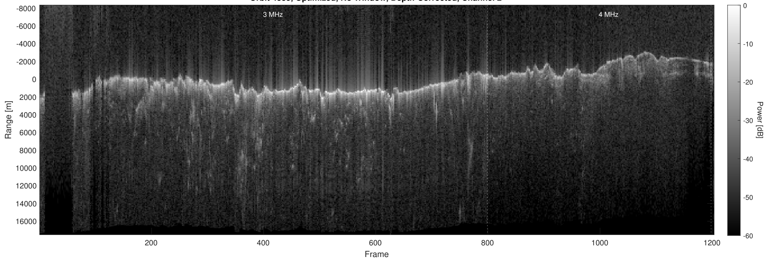
Orbit 4835, Optimized, No Window, Depth-Corrected, Channel 2
