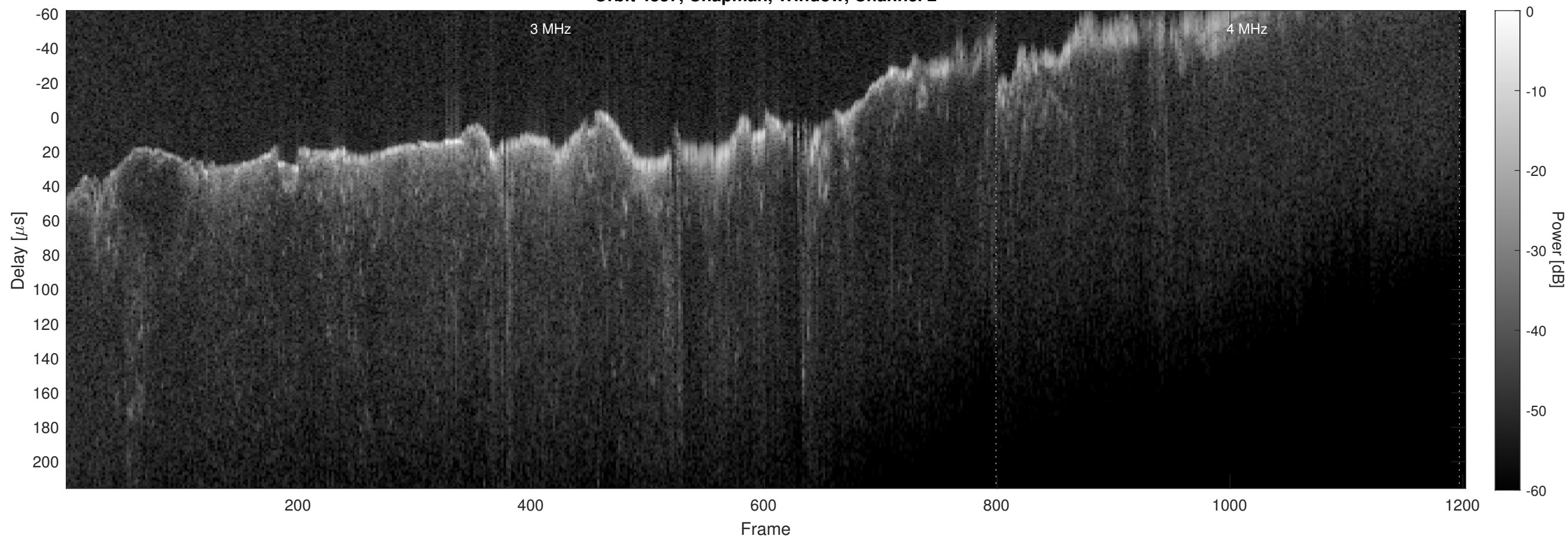
Orbit 4837, Chapman, Window, Channel 2
