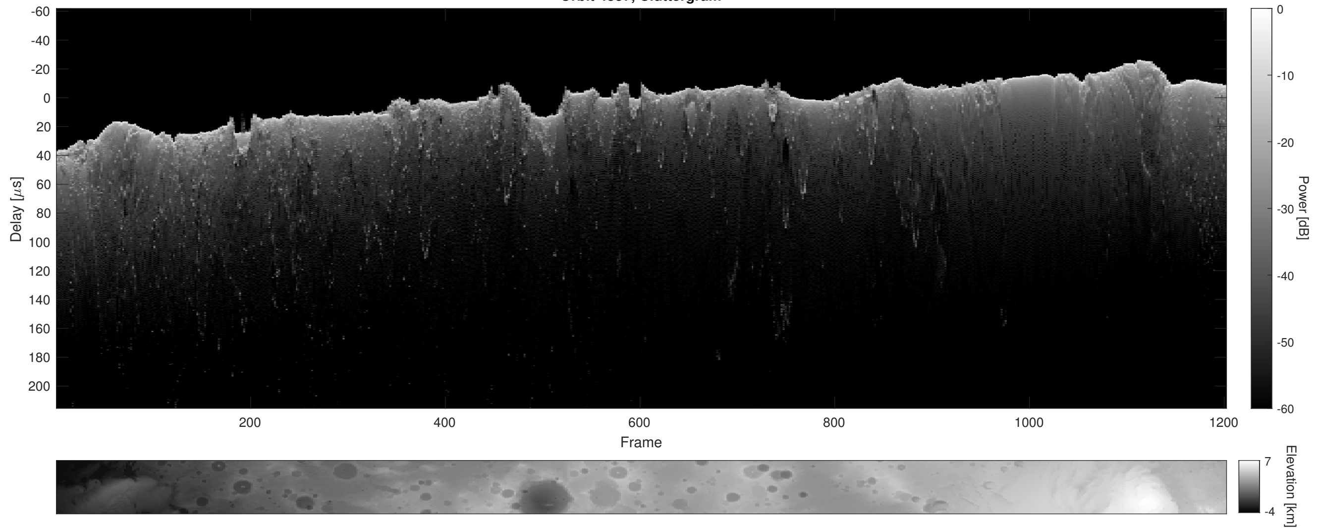
Orbit 4837, Cluttergram
