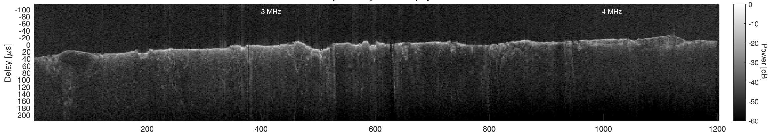
Orbit 4837, Cluttergram
