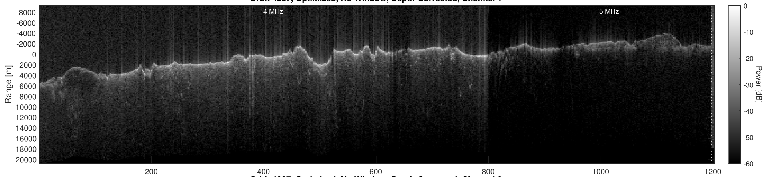
Orbit 4837, Optimized, No Window, Depth-Corrected, Channel 2
