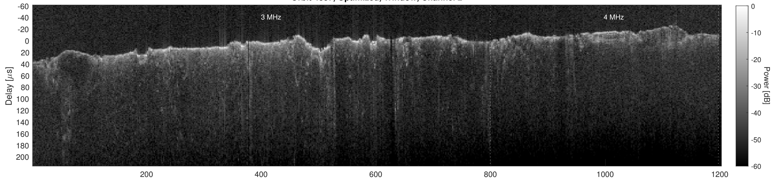
Orbit 4837, Cluttergram
