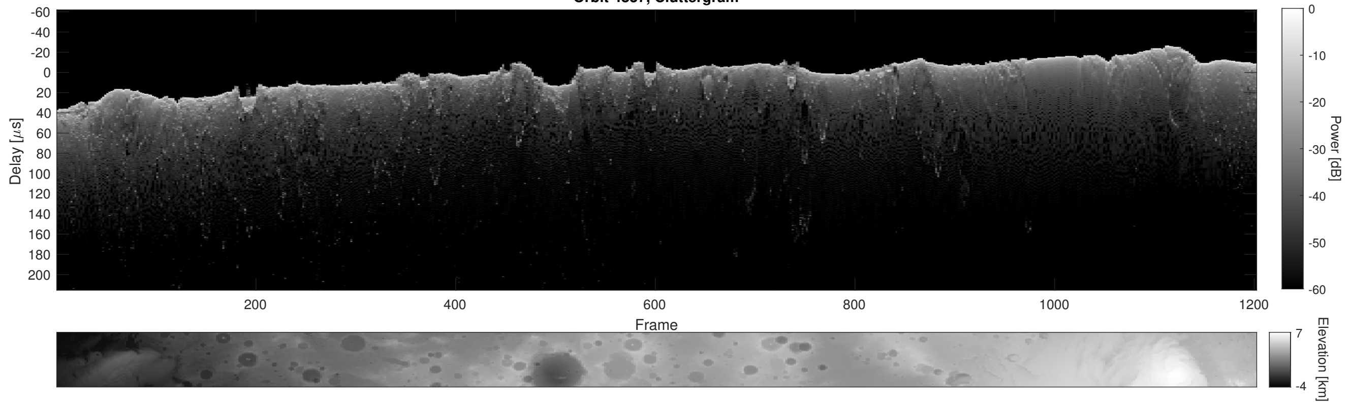
Orbit 4837, Cluttergram
