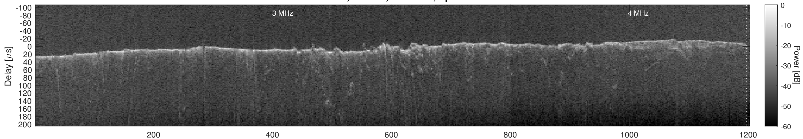
Orbit 4838, Cluttergram
