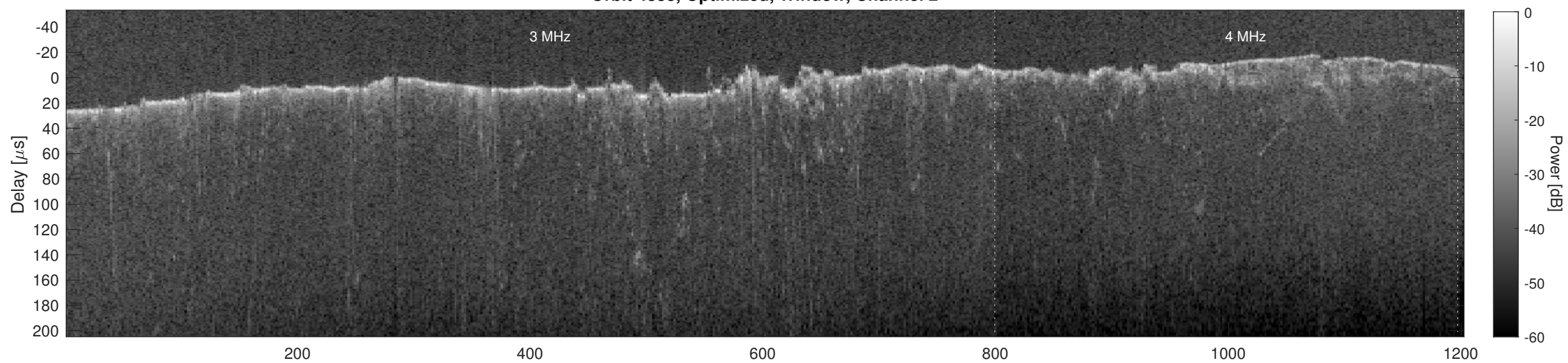
Orbit 4838, Cluttergram
