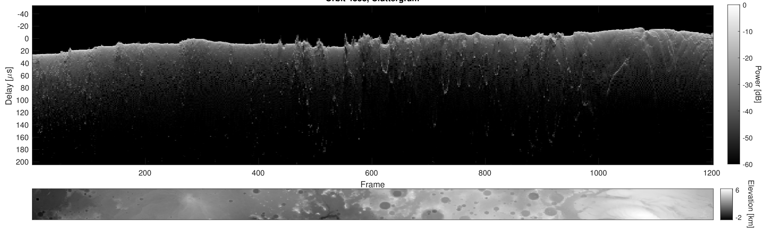
Orbit 4838, Cluttergram
