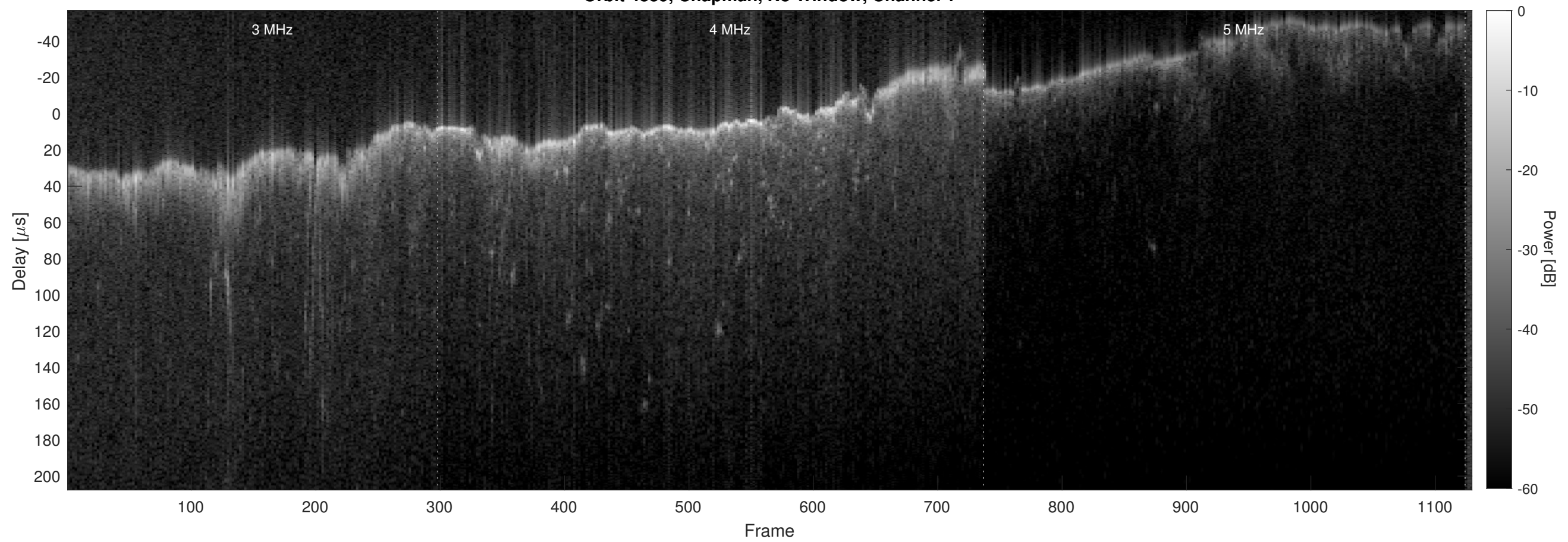
Orbit 4839, Chapman, No Window, Channel 2
