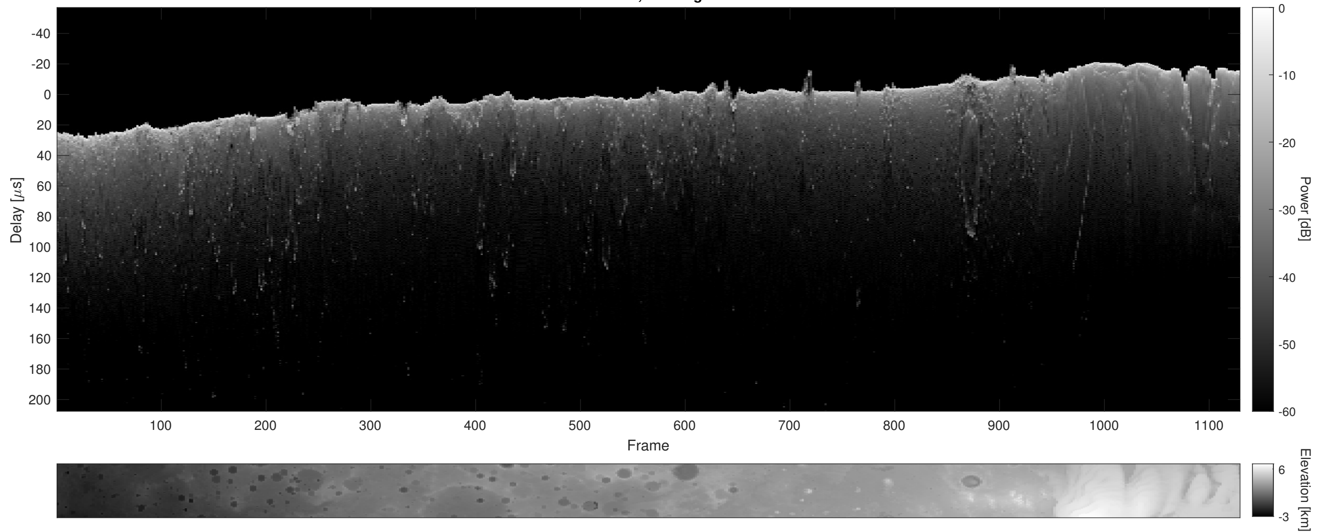
Orbit 4839, Cluttergram
