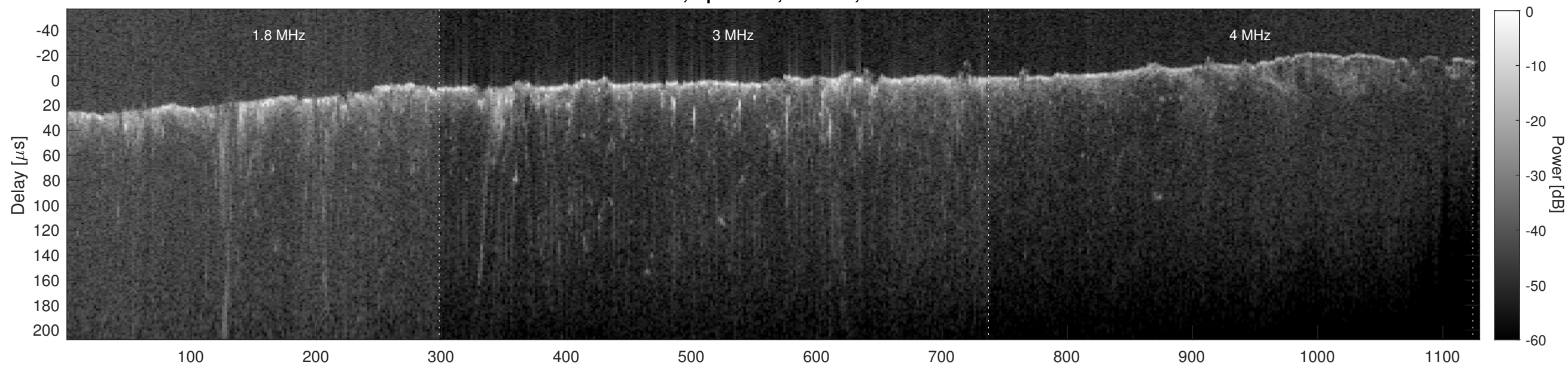
Orbit 4839, Cluttergram
