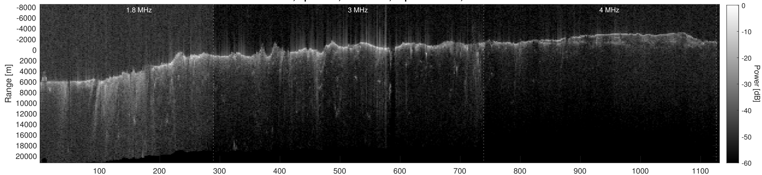
Orbit 4841, Depth-Corrected Cluttergram
