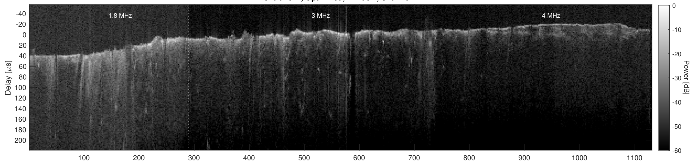
Orbit 4841, Cluttergram
