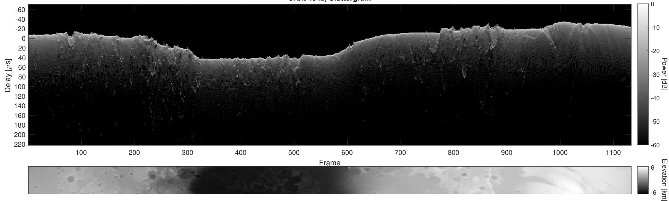
Orbit 4842, Cluttergram
