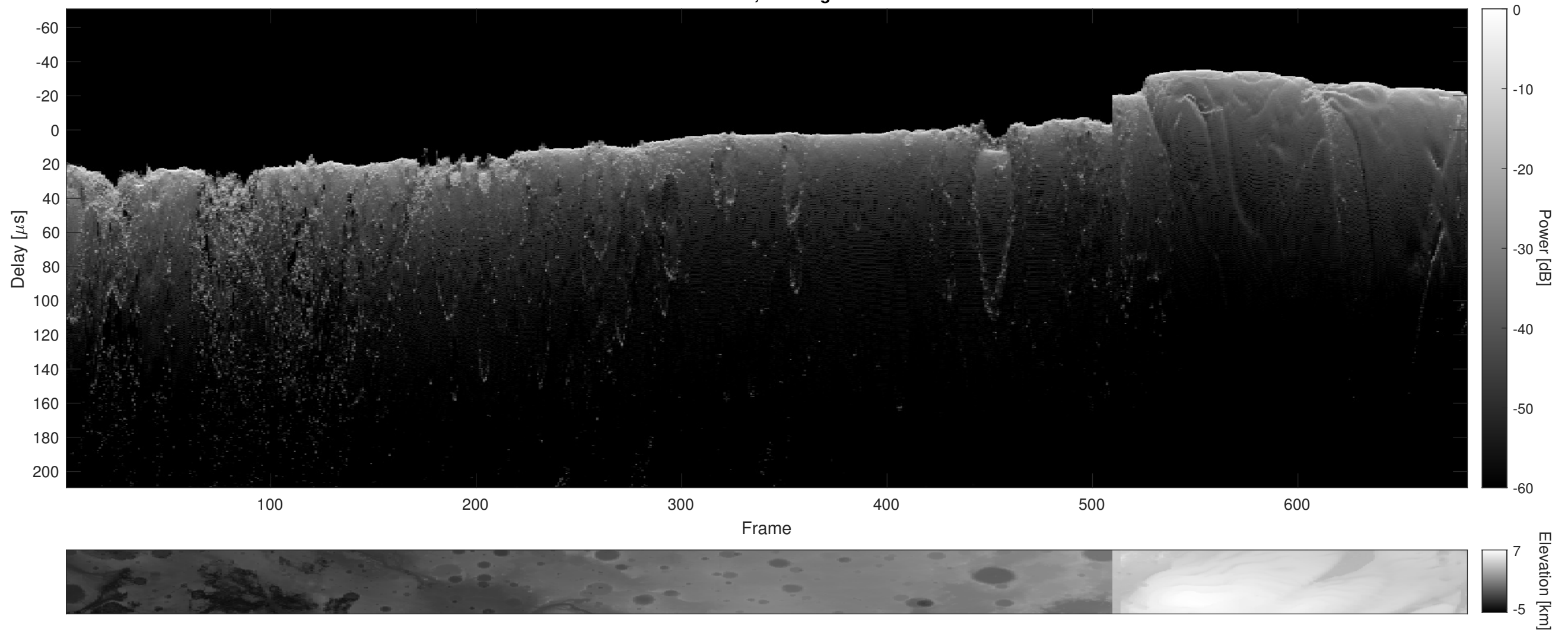
Orbit 4843, Cluttergram
