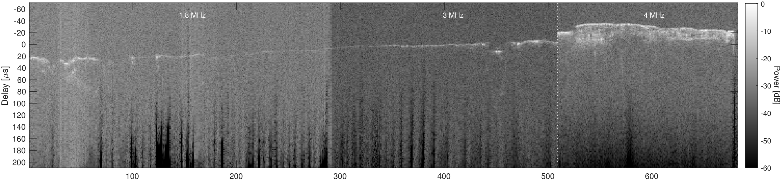
Orbit 4843, Cluttergram
