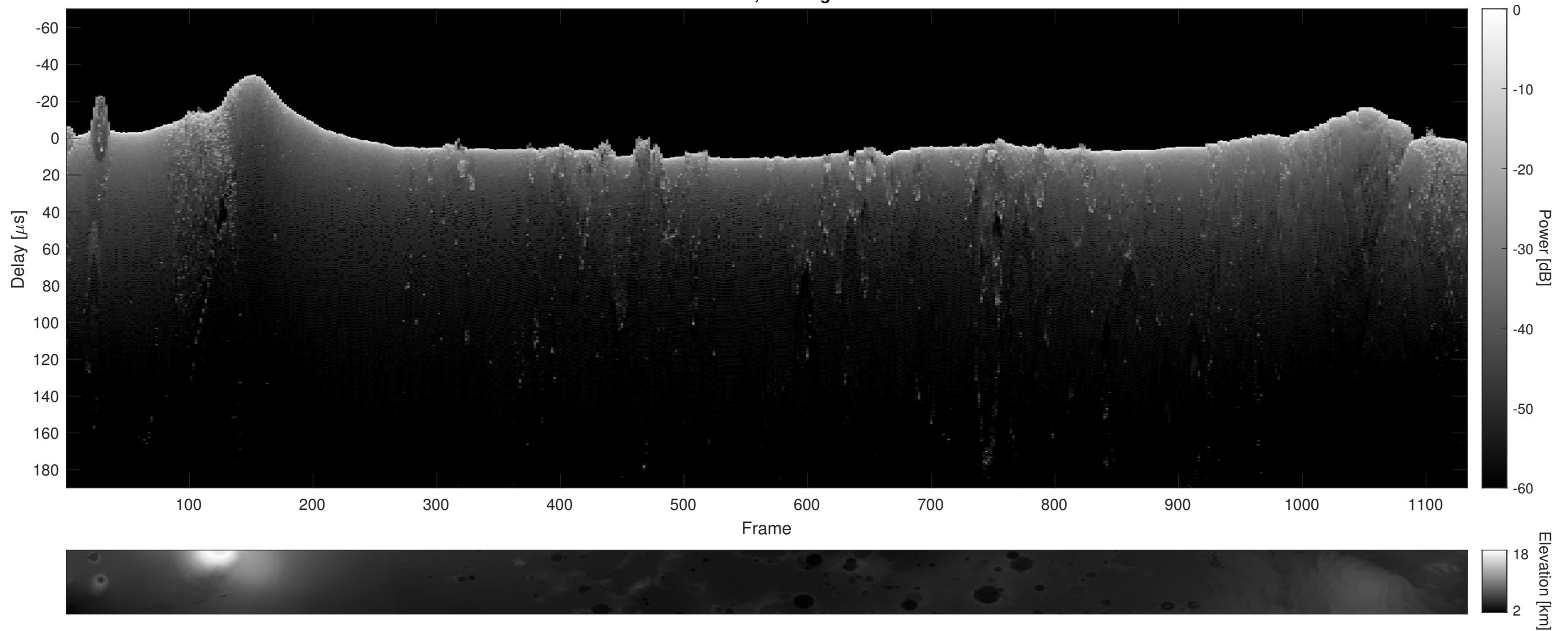
Orbit 4844, Cluttergram
