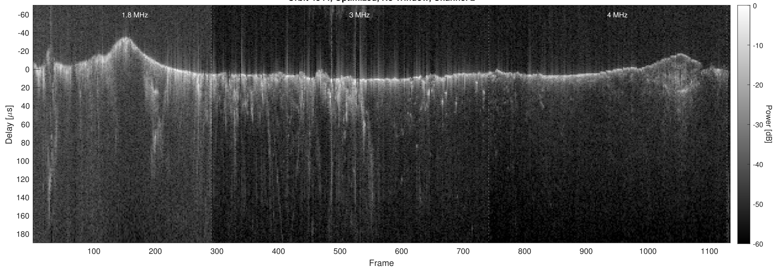
Orbit 4844, Optimized, No Window, Channel 2
