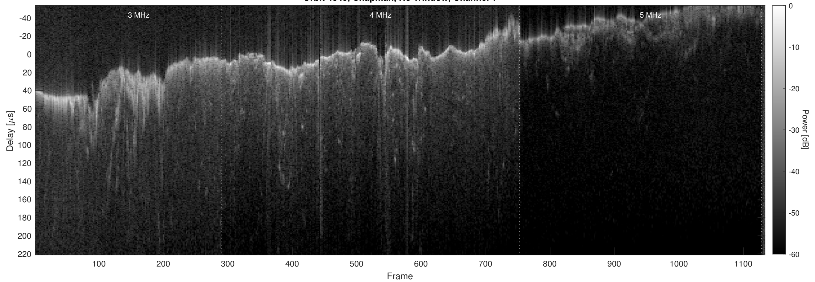
Orbit 4845, Chapman, No Window, Channel 2
