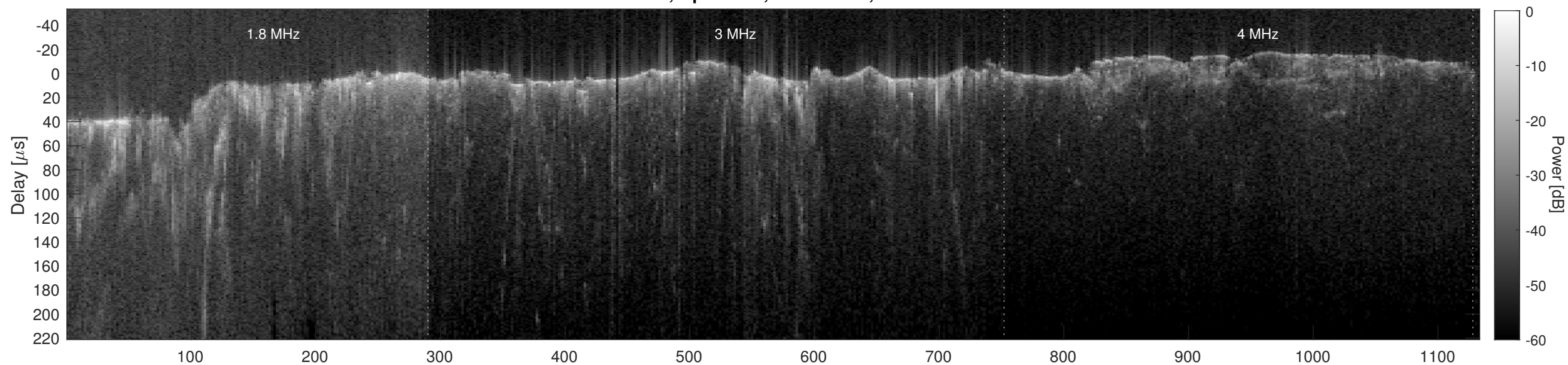
Orbit 4845, Cluttergram
