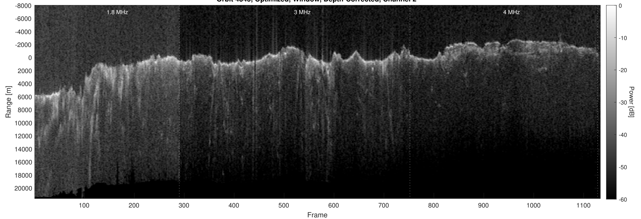
Orbit 4845, Optimized, Window, Depth-Corrected, Channel 2
