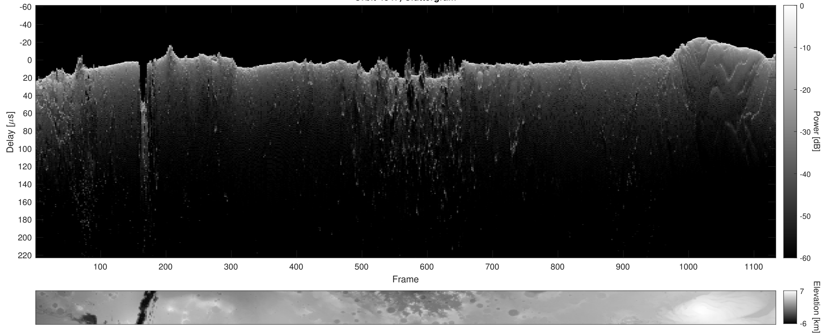
Orbit 4847, Cluttergram
