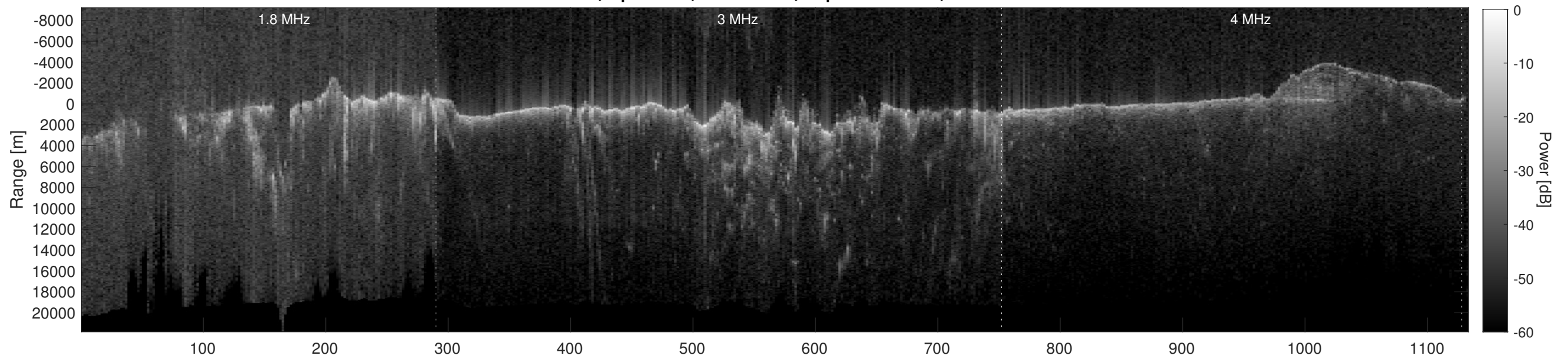
Orbit 4847, Depth-Corrected Cluttergram
