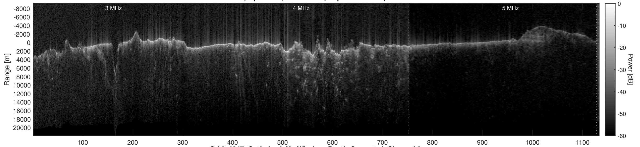
Orbit 4847, Optimized, No Window, Depth-Corrected, Channel 2
