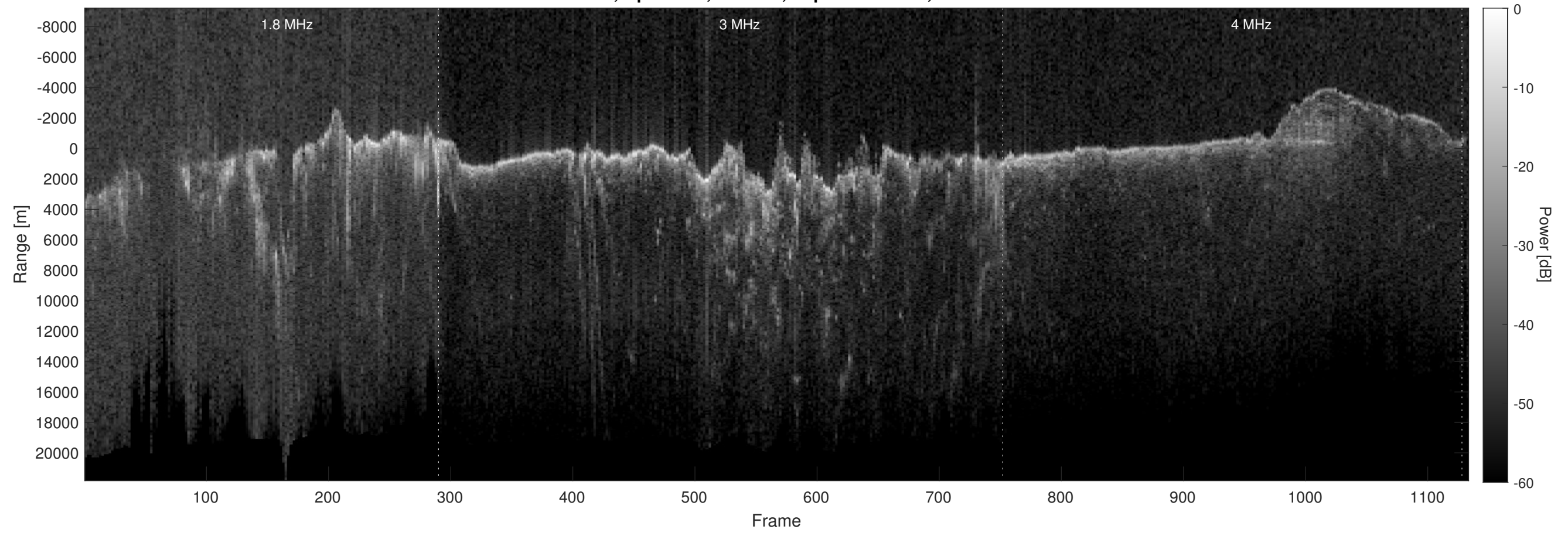
Orbit 4847, Optimized, Window, Depth-Corrected, Channel 2
