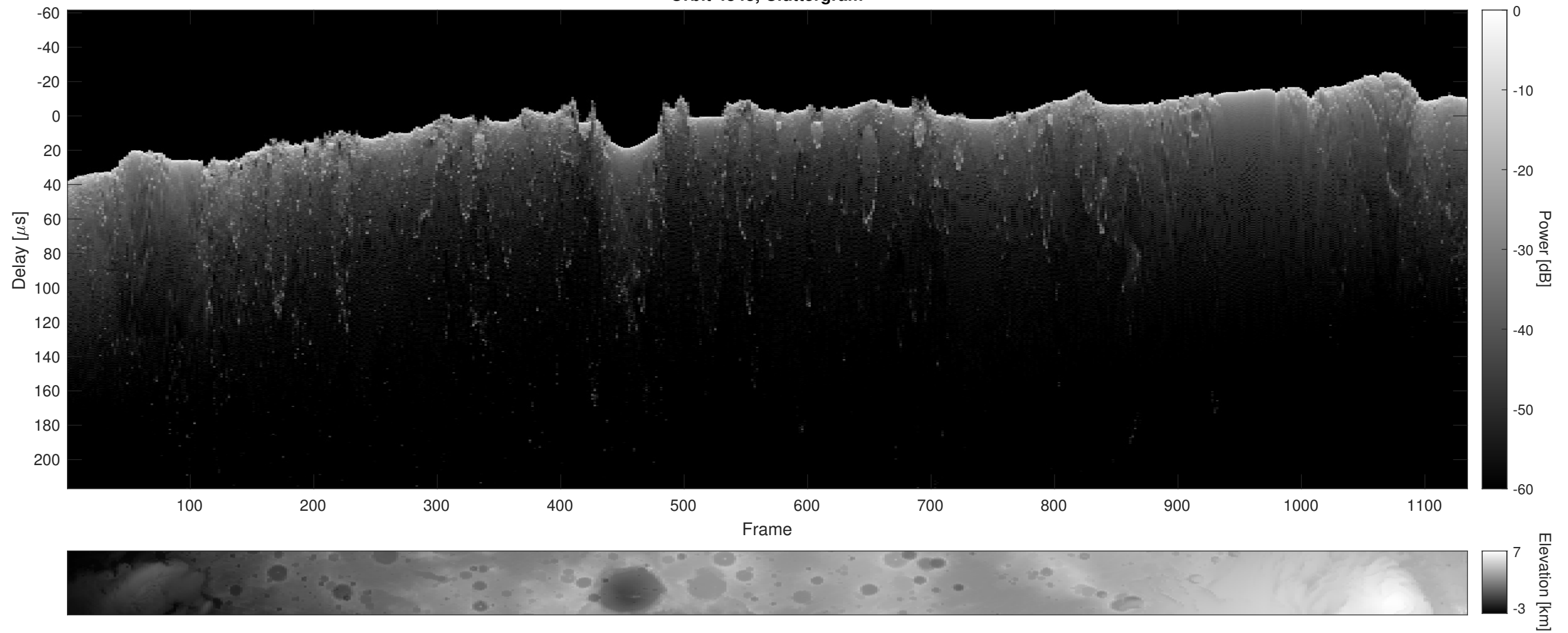
Orbit 4848, Cluttergram
