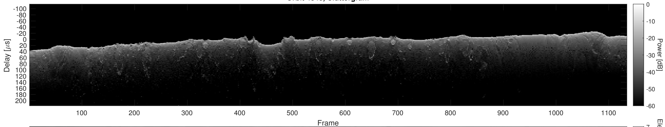
Orbit 4848, Cluttergram
