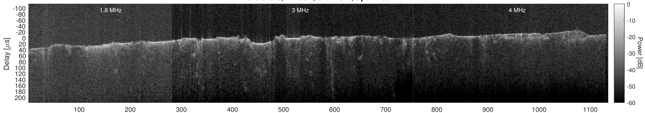
Orbit 4848, Cluttergram
