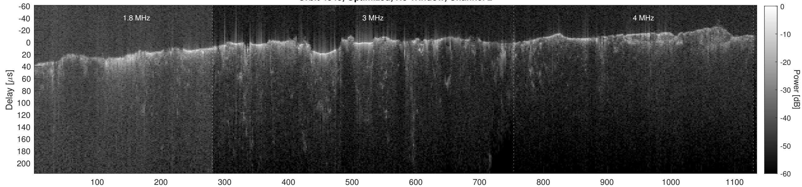
Orbit 4848, Cluttergram
