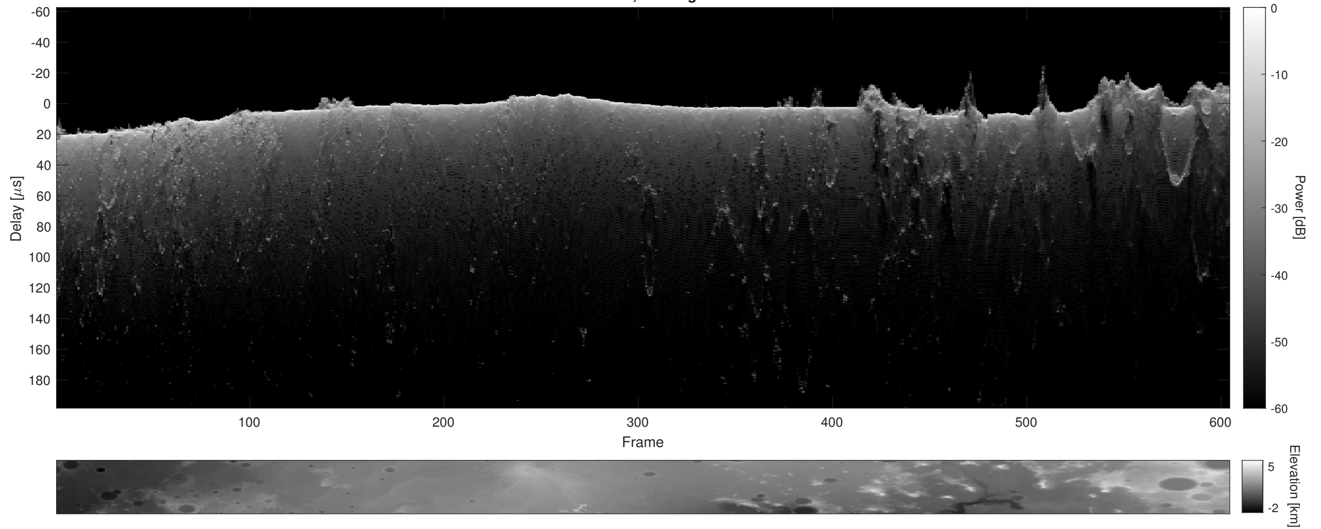
Orbit 4849, Cluttergram
