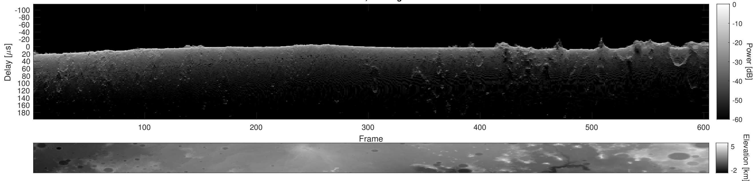
Orbit 4849, Cluttergram
