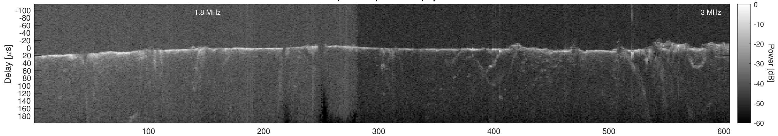
Orbit 4849, Cluttergram
