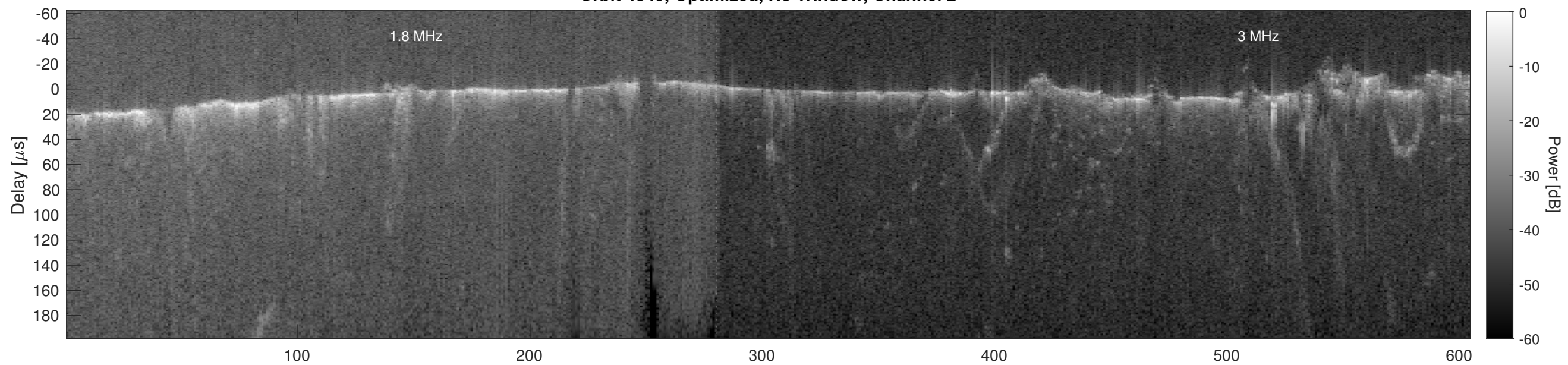
Orbit 4849, Cluttergram
