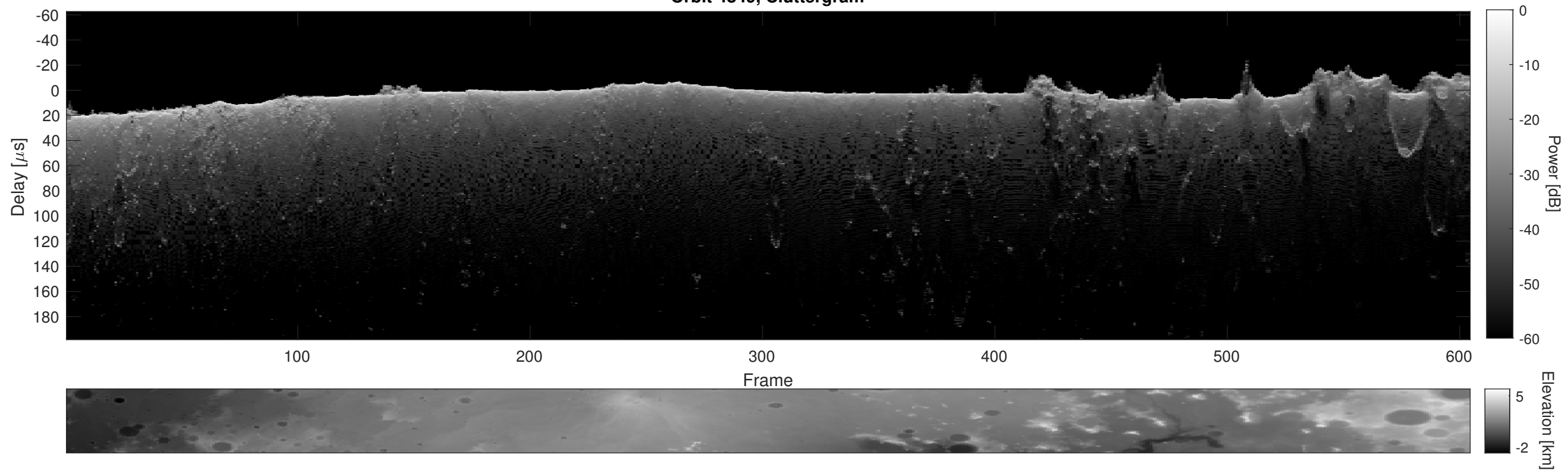
Orbit 4849, Cluttergram
