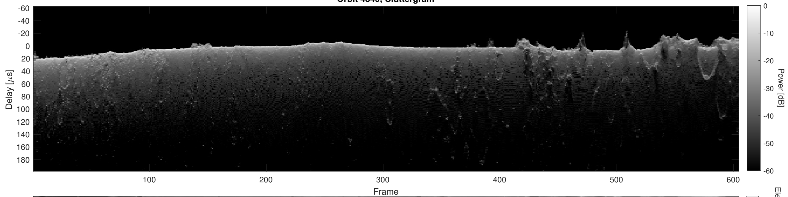
Orbit 4849, Cluttergram
