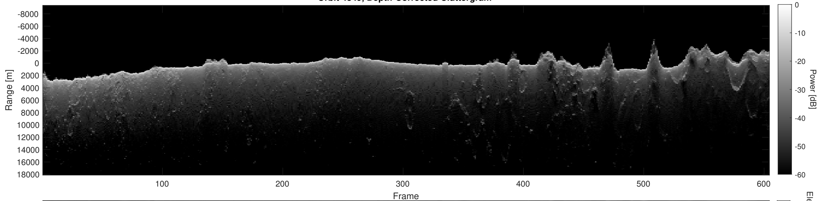
Orbit 4849, Depth-Corrected Cluttergram
