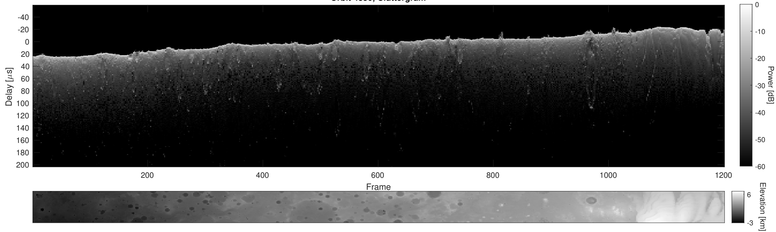
Orbit 4850, Cluttergram
