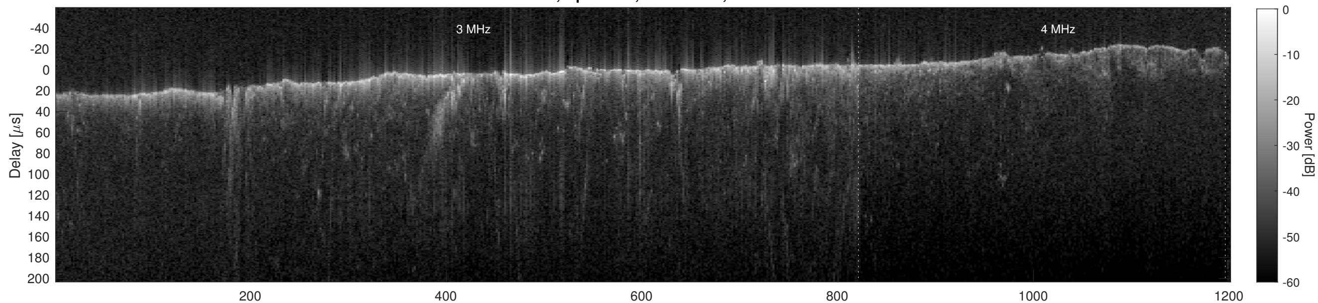
Orbit 4850, Cluttergram
