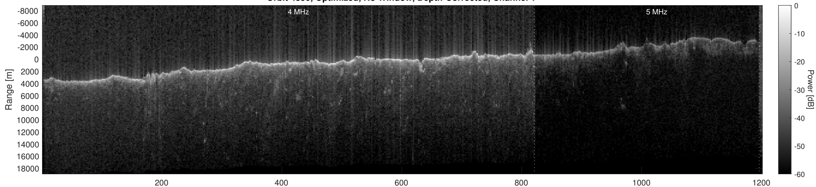
Orbit 4850, Optimized, No Window, Depth-Corrected, Channel 2
