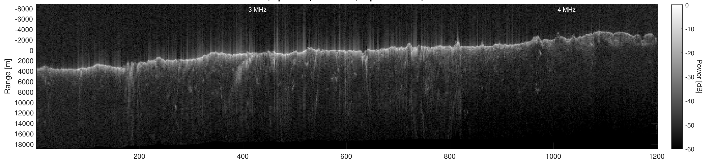
Orbit 4850, Depth-Corrected Cluttergram
