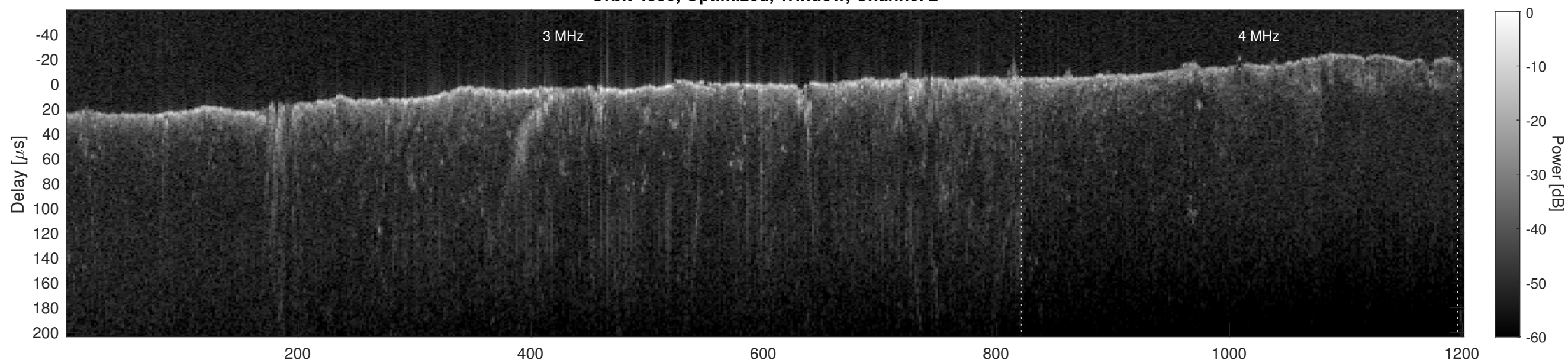
Orbit 4850, Cluttergram
