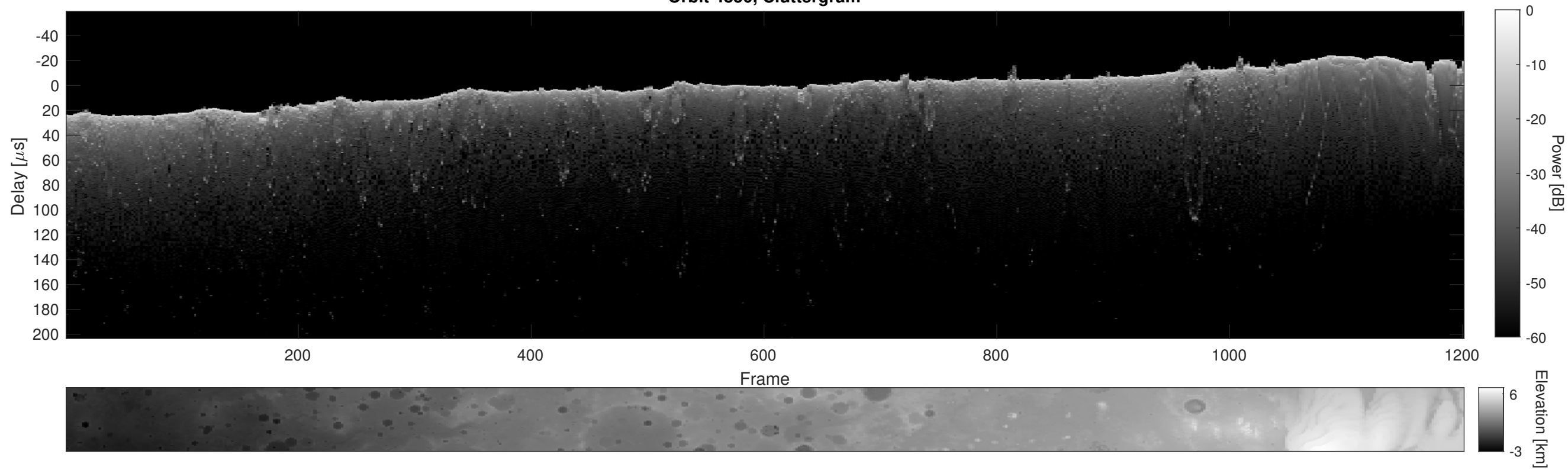
Orbit 4850, Cluttergram
