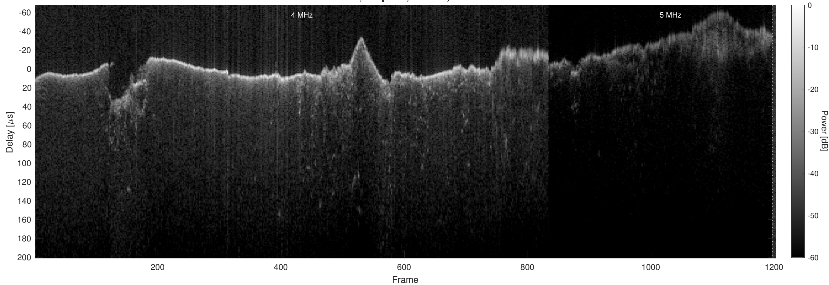
Orbit 4851, Chapman, Window, Channel 2
