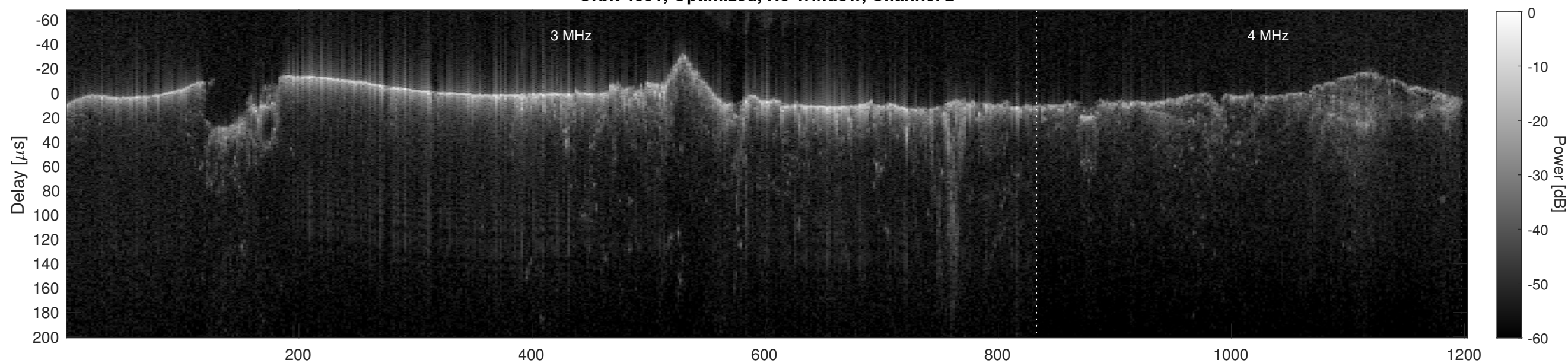
Orbit 4851, Cluttergram
